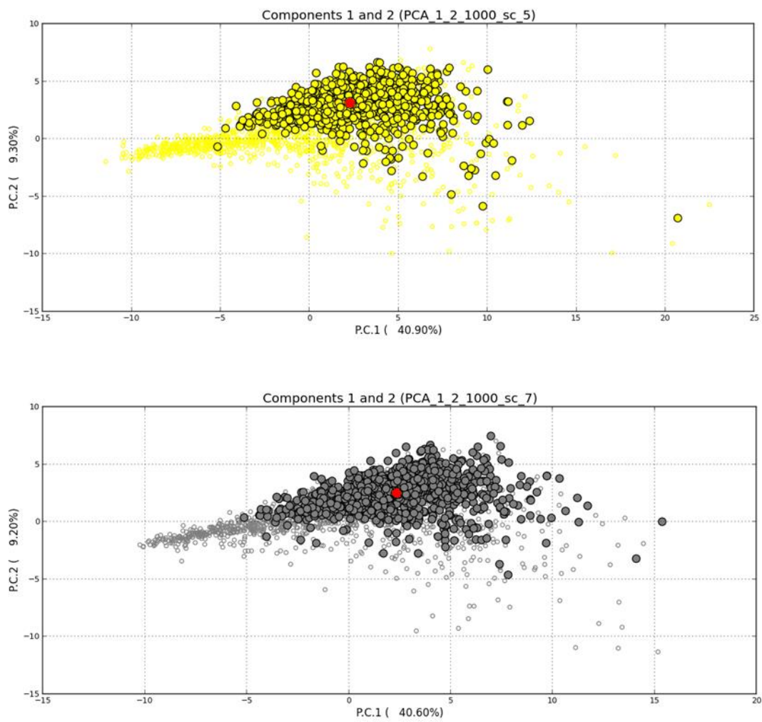
Fig. S4 PCA summary statistics simulated under the most probable scenarios: Scenario 5 (atop) and 7 (bottom). Small circles correspond to simulated statistics from the prior, the large dots correspond to the simulated posteriors and the red dot represents the real data set.
