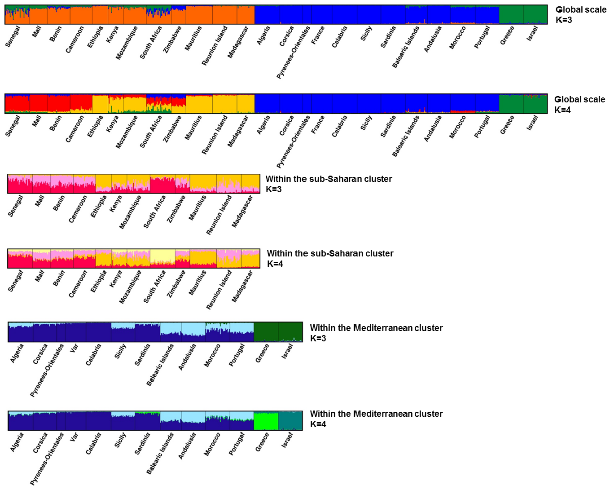
Fig. S2 Ancestry estimation assuming three and four population clusters (K=3 and K=4) based on the Bayesian clustering method implemented in STRUCTURE v.2.3.3. Each vertical line represents an individual, and each color represents a cluster. Individuals are grouped by sample site.
